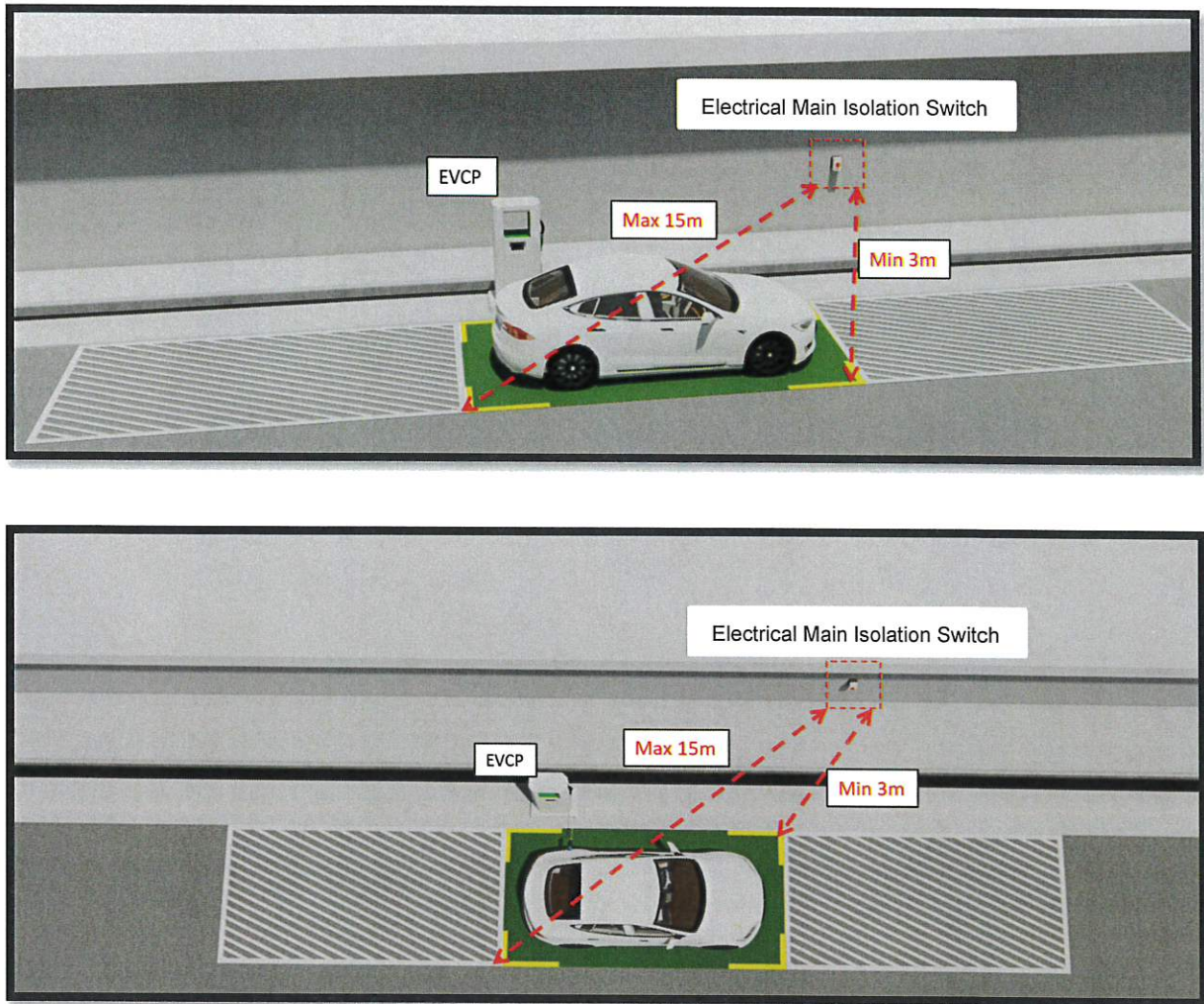
Gambar Rajah 1 :Penempatan Electrical Main Isolation Switch
